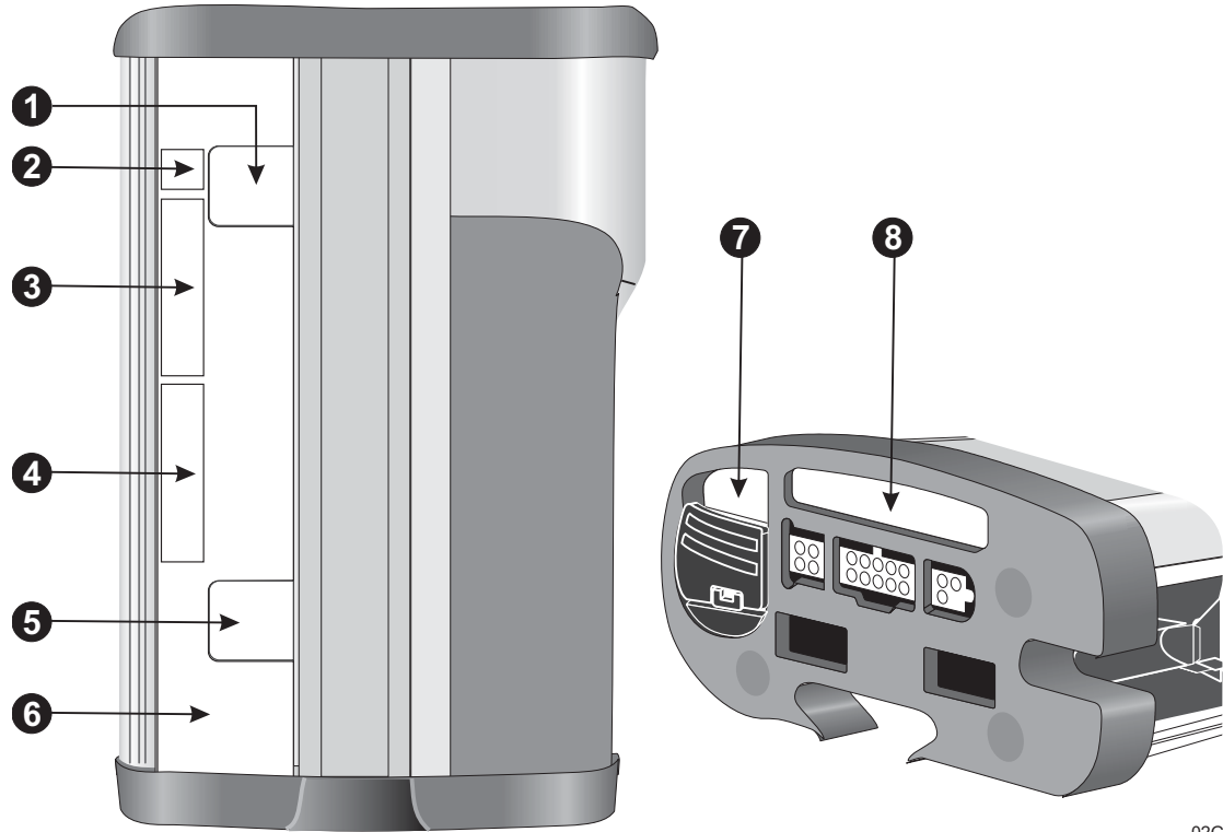
Figure 5-2. Label Inspection
