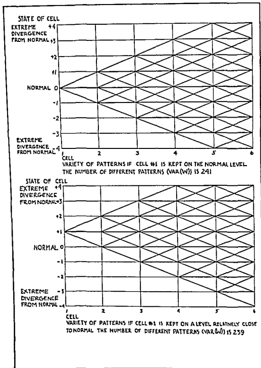
FIGURE 73. The effect on the variety of possible patterns of restricting the level of cell 1 to two different levels.
