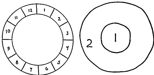
FIGURE 69 Degree of centrality. The diagram at the left represents a whole containing 12 peripheral cells, dif(W) = 12 , cent(x) = const = 0 , cen\ str(W) = 1 , inn\ str(W) = 1 . The diagram at the right represents a whole containing 2 peripheral cells, one of them being an inner cell, dif(W) = 2 , cent(1) = cent(2) = 0 , cen\ str(W) = 1 , inn(1) = 1 , inn(2) = 2 , inn\ str(W) = 2 .
